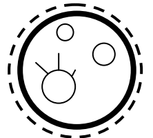
Mercury
