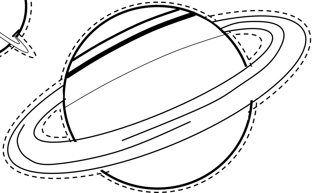
Saturn
